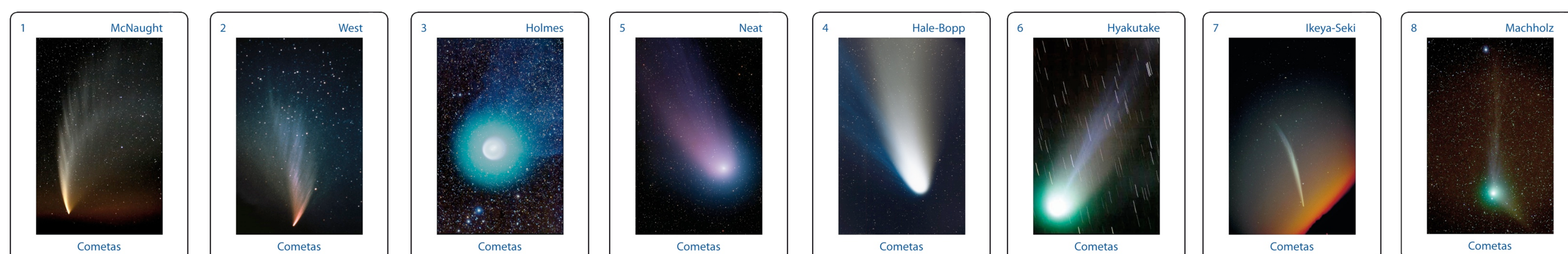
Comets
