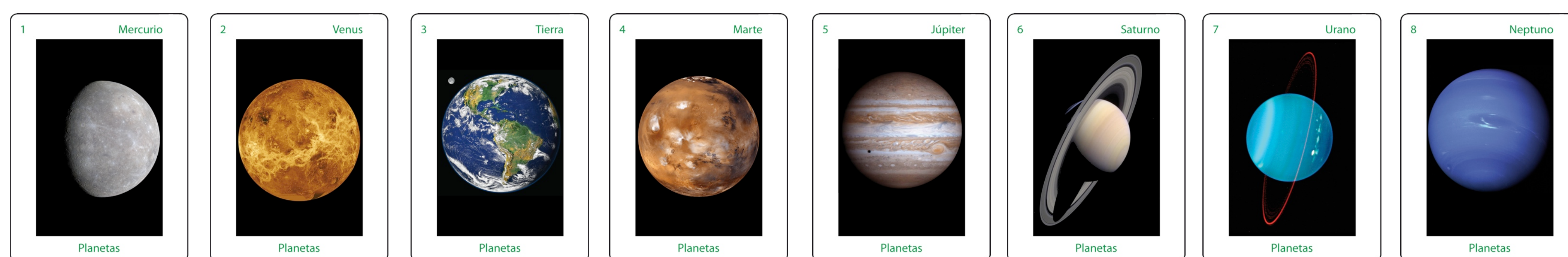
Planets
