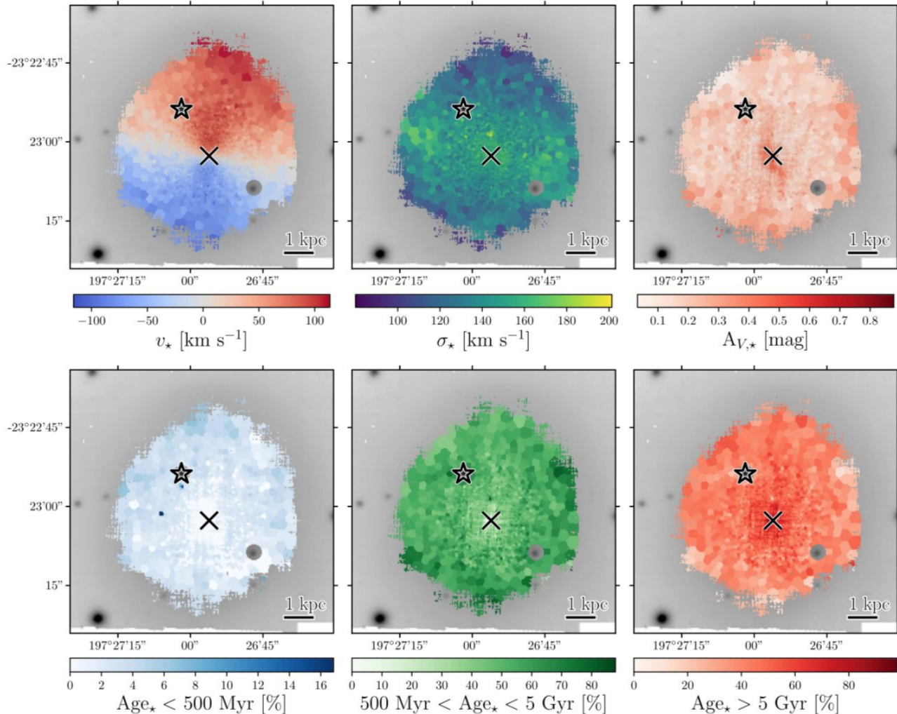
Figure 6. Stellar population map for NGC 4993 obtained with MUSE (Levan et al. 2017). The upper panels show the distribution of the radial velocities (left) as estimated from the stellar components for each single spectral bin, as well as its dispersion in terms of \sigma (middle) and the extinction as inferred from the fit continuum (right). Lower panels show the distribution of stellar ages for different age intervals: less than 500 Myr (left), between 500 Myr and 5 Gyr (middle) and larger than 5 Gyr (right). The black star corresponds to the location of the kilonova AT2017gfo.
